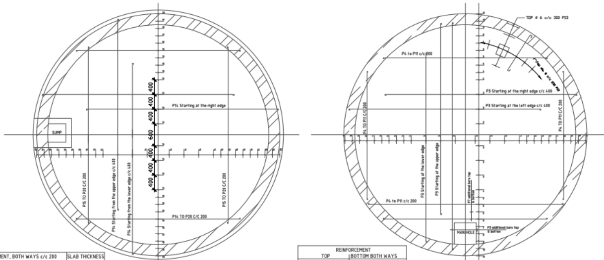
FLOOR REINFORCEMENT SCALE 1:50
